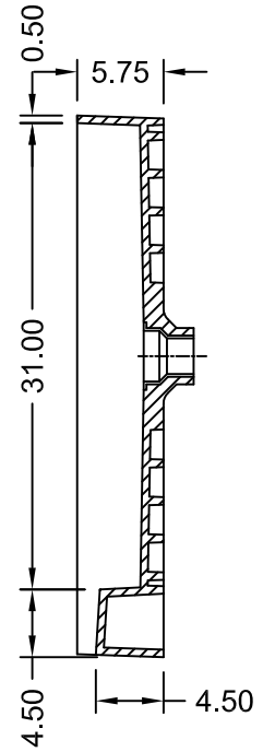
SECTION B-B
